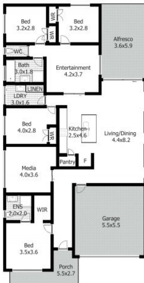
FLOOR PLAN
